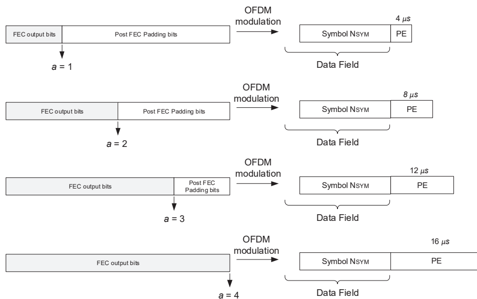
Figure 27-44—PE field duration of an HE SU PPDU or HE ER SU PPDU without midambles if TXVECTOR parameter NOMINAL\_PACKET\_PADDING is 16 \mu s and T_{PE} = T_{PE,nominal}
