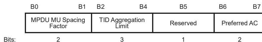
Figure 9-64g—Trigger Dependent User Info subfield format in the Basic Trigger frame
