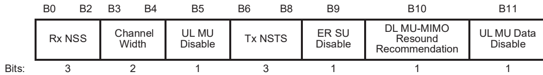
Figure 9-22b—Control Information subfield format in an OM Control subfield
