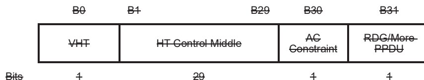
Figure 9-11—Non-CMMG variant HT Control field format
