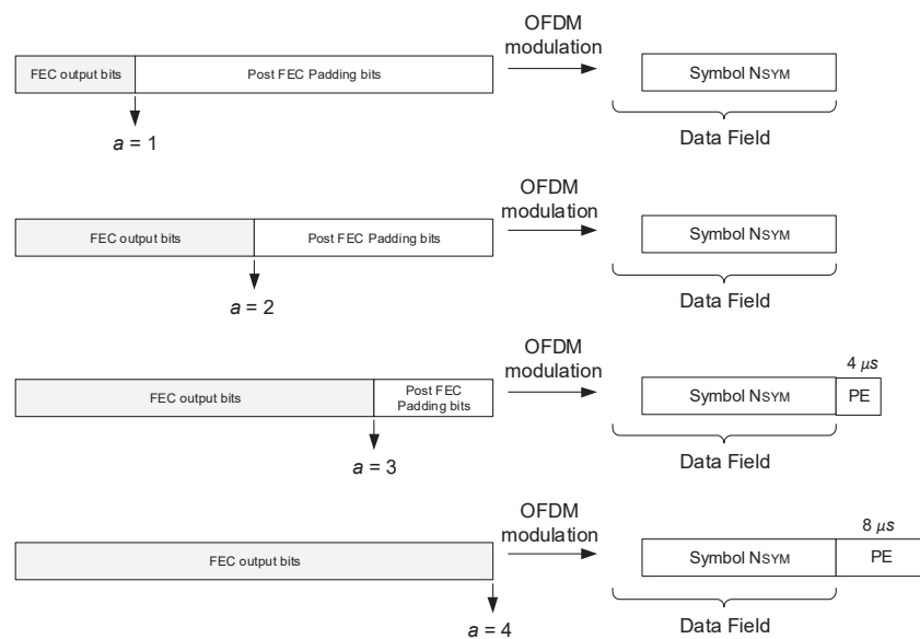
Figure 27-43—PE field duration of an HE SU PPDU or HE ER SU PPDU without midambles if TXVECTOR parameter NOMINAL\_PACKET\_PADDING is 8 \mu s and T_{PE} = T_{PE,nominal}
