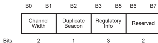
Figure 9-788l—Control field format
