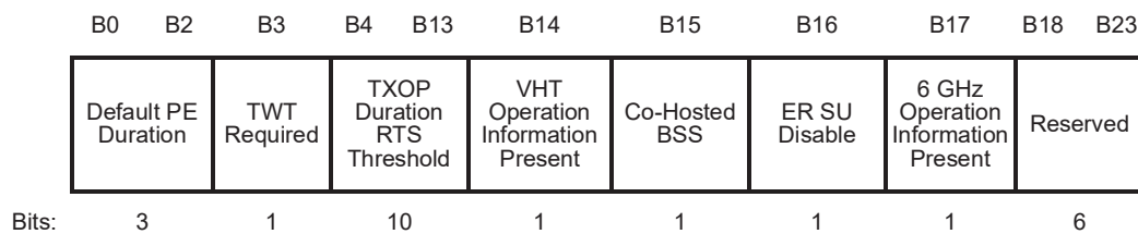
Figure 9-788i—HE Operation Parameters field format
