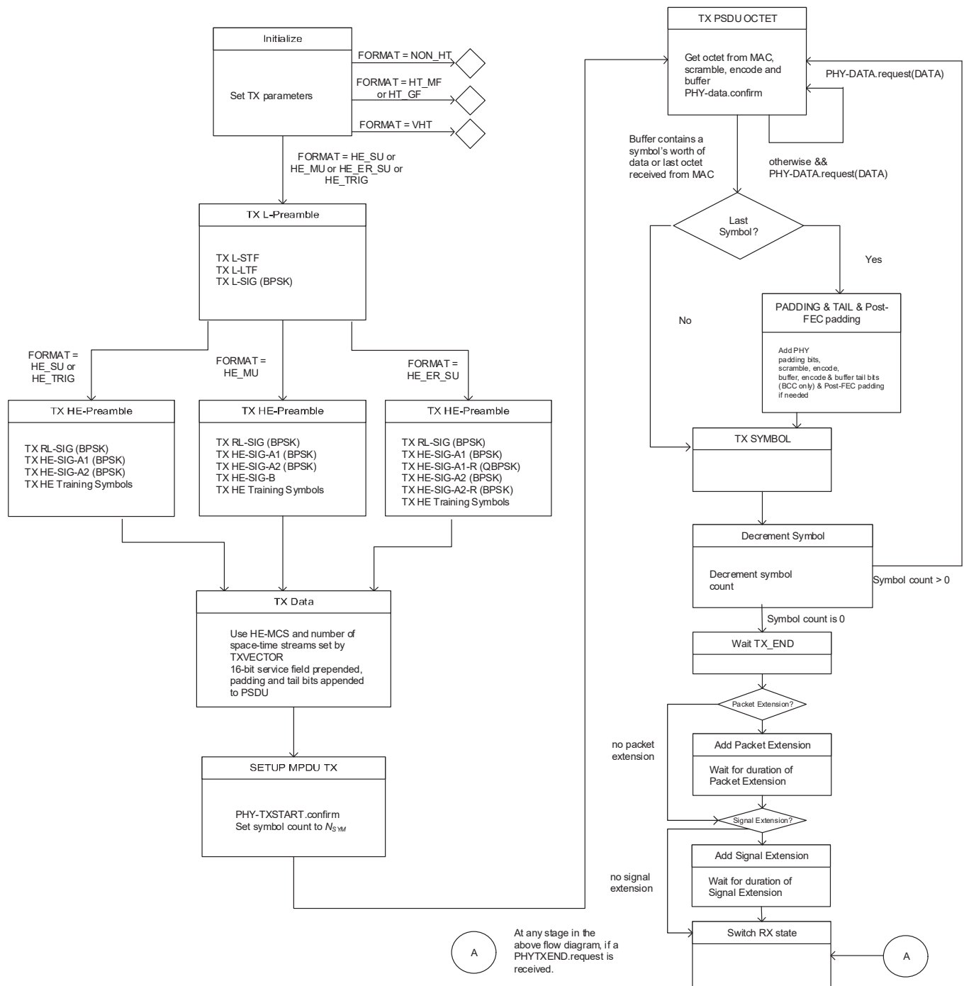
Figure 27-58—PHY transmit state machine for an HE PPDU without midambles
