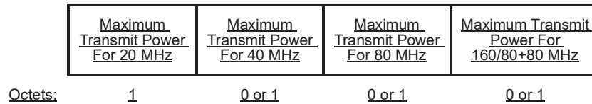
Figure 9-617a—Maximum Transmit Power field format if the Maximum Transmit Power Interpretation subfield is 0 or 2
