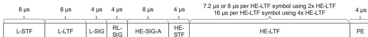
Figure 27-45—HE sounding NDP format
